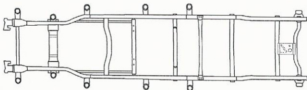
UNDERBODY VIEW
